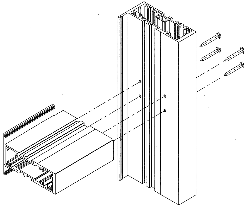
INTERMEDIATE HORIZONTAL CORNERS
