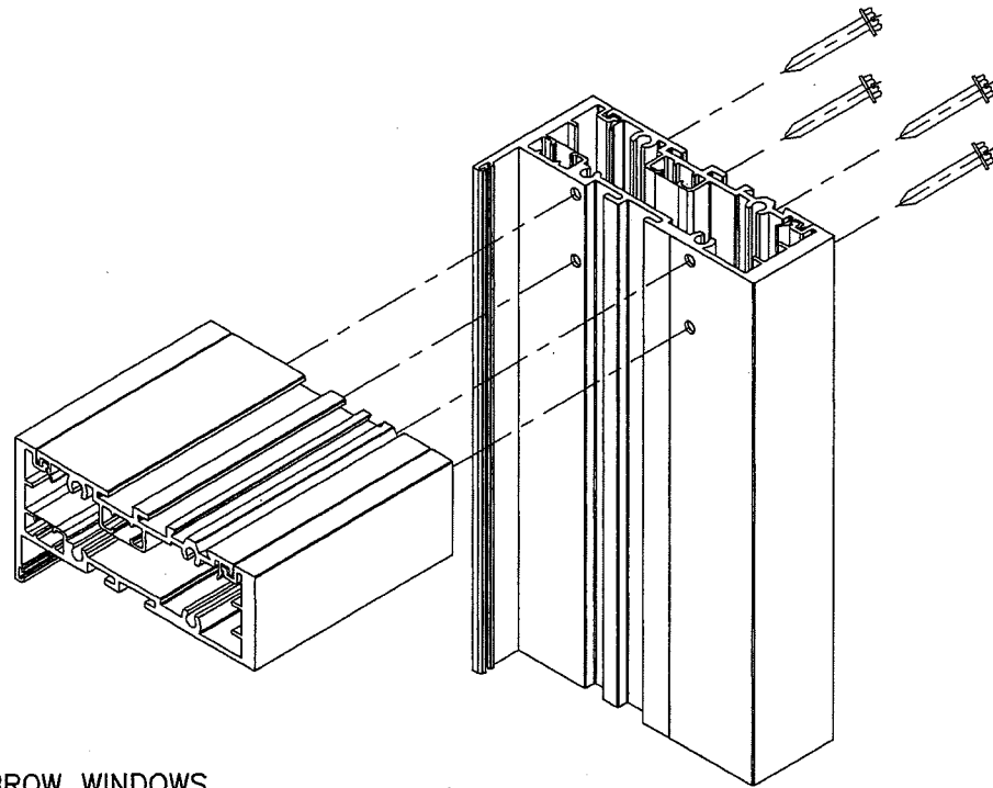
FRAME TOP/BOTTOM CORNERS
