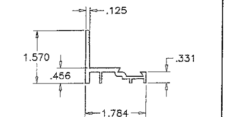
EXTERIOR GLASS STOP (DOOR)
