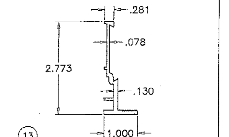
EXTERIOR GLASS STOP (TRANSOM)
