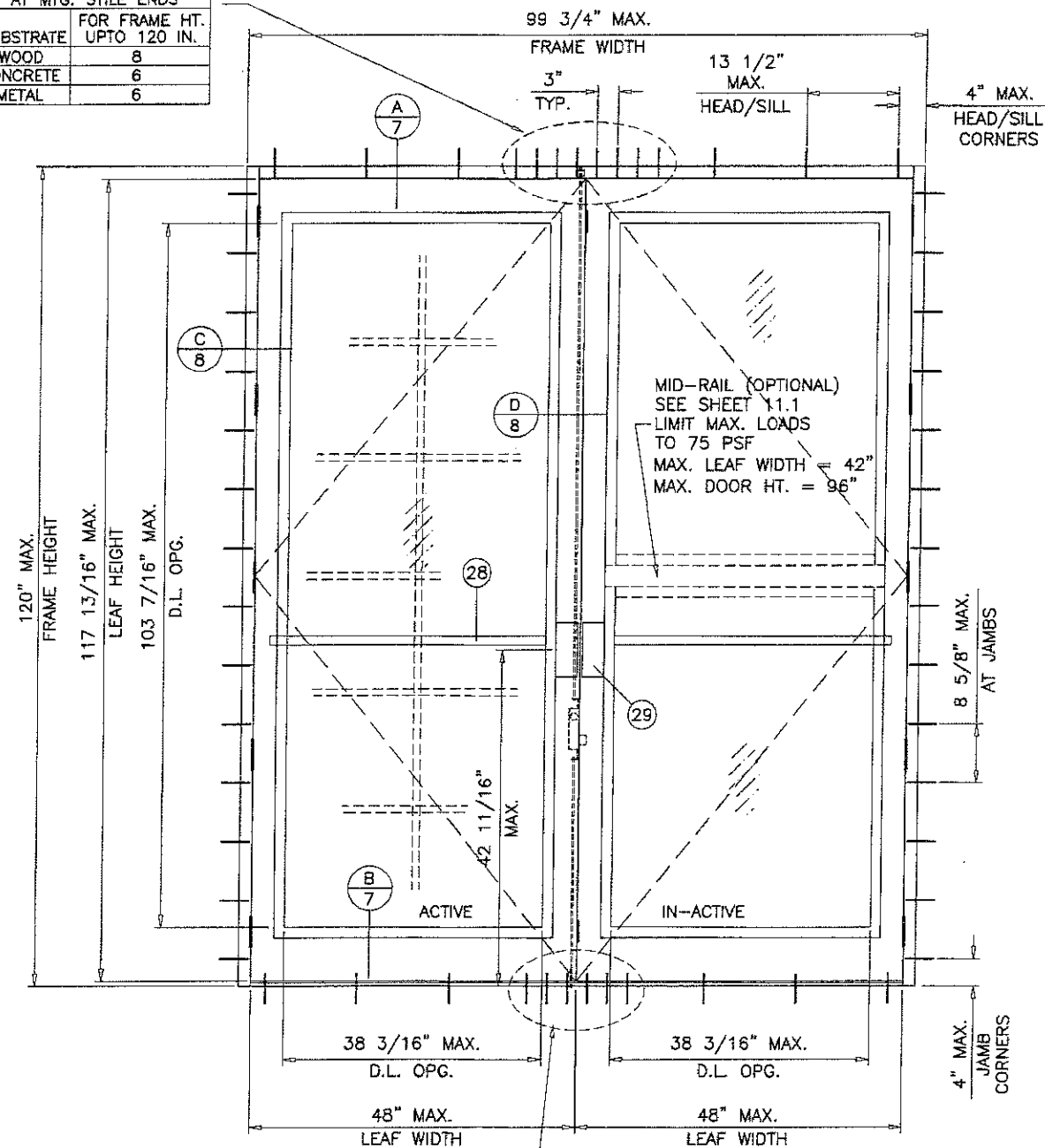
TYPICAL ELEVATIONS
