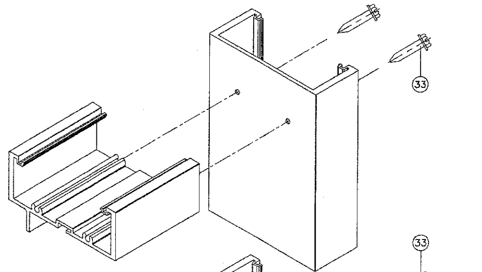
FRAME TOP CORNER
