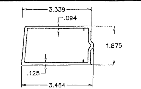
DOOR STILE
