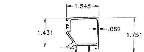
HI-RISE THRESHOLD COVER
