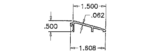
THRESHOLD RAMP ADAPTER
