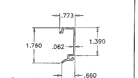
INTERIOR GLASS STOP (TRANSOM)
