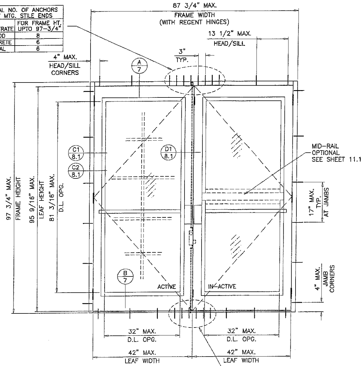
( XX ) TYPICAL ELEVATION
