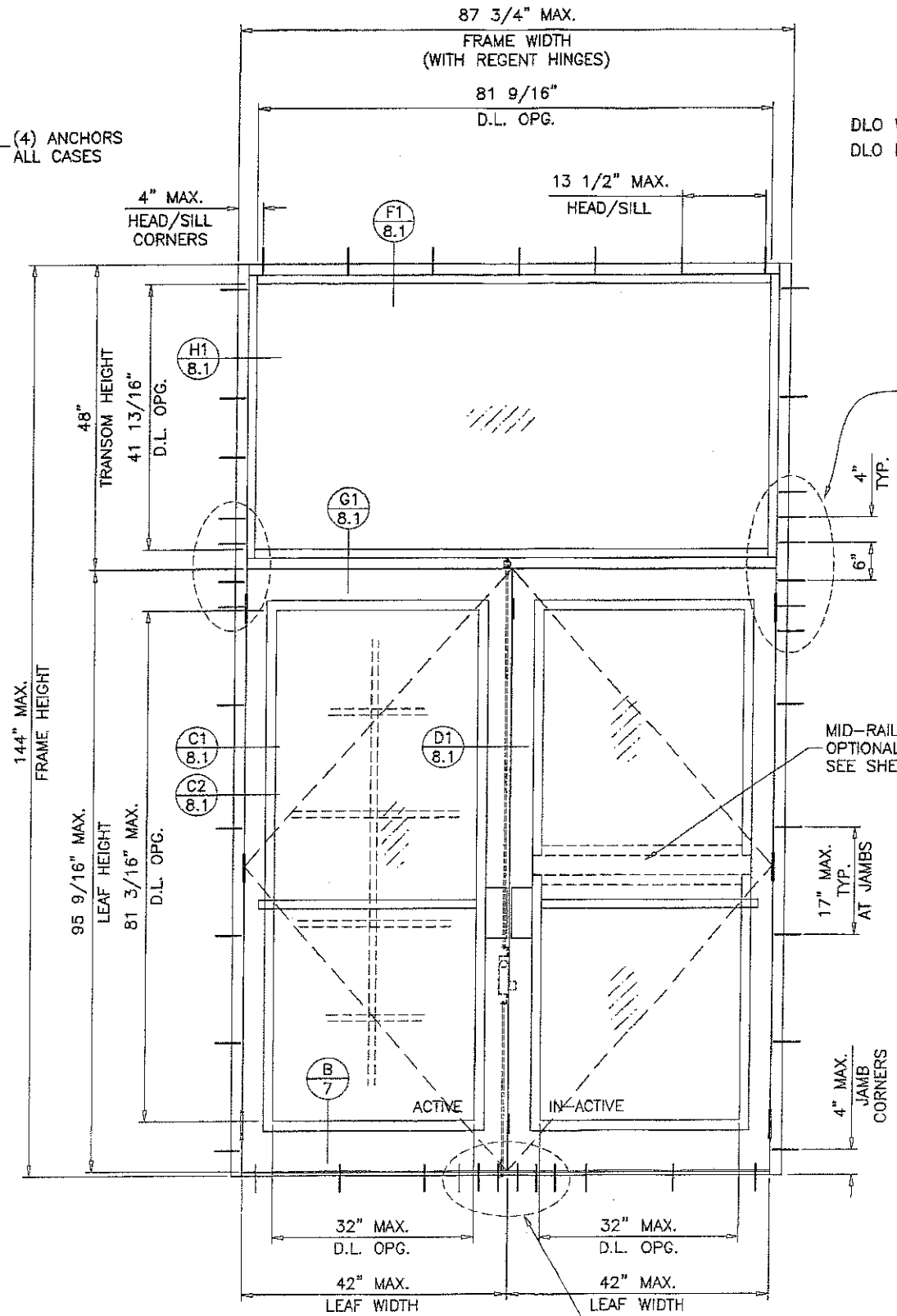
( O/XX ) TYPICAL ELEVATION
