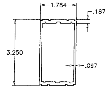
4 MID-RAIL
