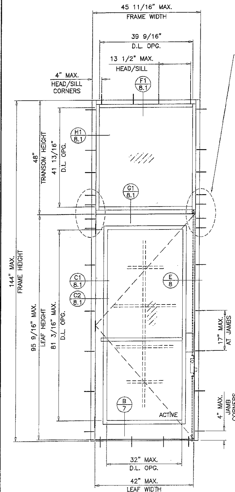
( O/X ) TYPICAL ELEVATION
