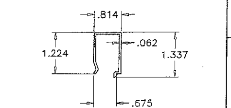
INTERIOR GLASS STOP (DOOR)
