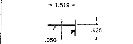
DOOR STOP COVER
