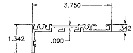
13.1 TRANSOM ADAPTER
