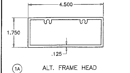
FRAME HEAD
