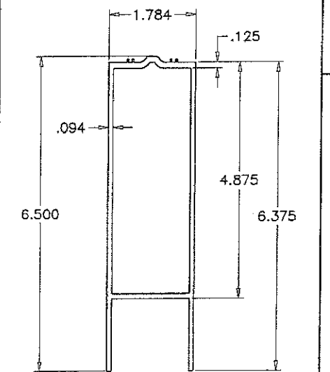
BOTTOM RAIL
