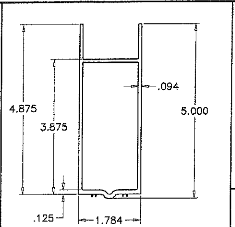
TOP RAIL
