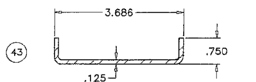
REINFORCING CHANNELS
