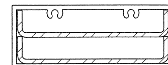
TRANSOM BAR HORIZONTAL MULLION WITH REINFORCING
