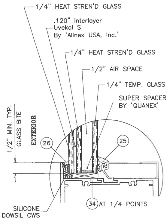
GLASS TYPE 'G7'
