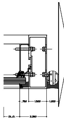
UNANCHORED JAMB OPTION DETAIL OF FRONTSET PLUS MONUMENTAL WITH LAMINATED GLASS.
