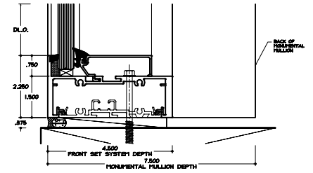
SILL DETAIL OF FRONTSET PLUS MONUMENTAL WITH LAMINATED GLASS.
