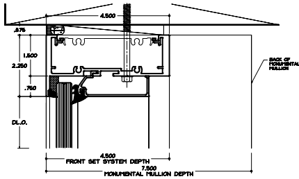
HEAD DETAIL OF FRONTSET PLUS MONUMENTAL WITH LAMINATED GLASS.
