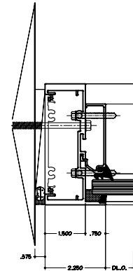
ANCHORED JAMB DETAIL OF FRONTSET PLUS MONUMENTAL WITH LAMINATED GLASS.
