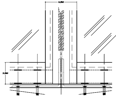
EXTERIOR VIEW OF FRONTSET PLUS MONUMENTAL WITH LAMINATED GLASS.
