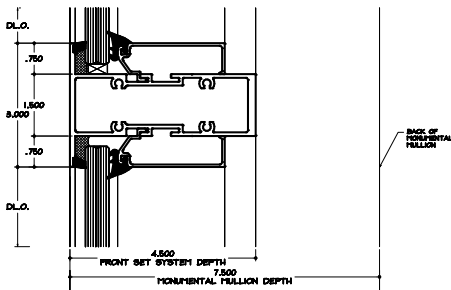
INTERMEDIATE HORIZONTAL DETAIL OF FRONTSET PLUS MONUMENTAL WITH LAMINATED GLASS.
